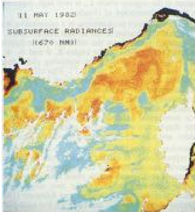
Figure 4 in: Bricaud, A., and A. Morel (1987). Atmospheric corrections and interpretation of marine radiances in CZCS imagery: use of a reflectance model. Oceanologica Acta , N°SP, 33-50.
