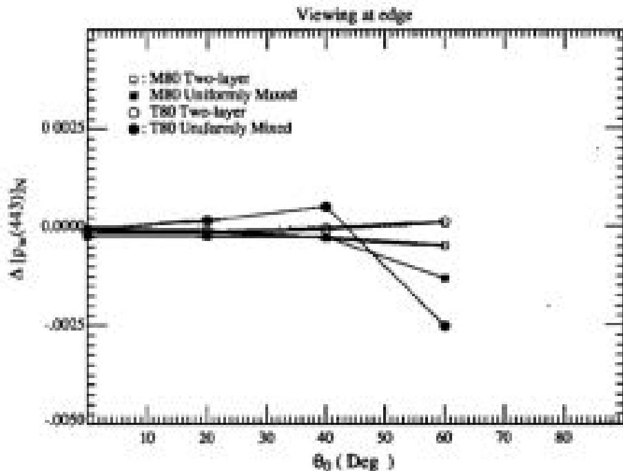
Figure 14a. Effect of the vertical distribution of aerosol on \Delta[\rho_w(443)]_w as a function of \theta_0 at the edge of the scan for the T80 and M80 aerosol models with \tau_a(865) = 0.2 . Note that the correction algorithm assumes that the “two-layer” stratification is correct.
