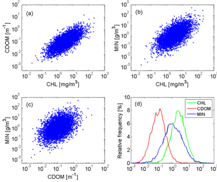
Figure 4.1 Covariation and distribution of CHL, MIN and CDOM in the CCRR synthetic dataset. Panels (a), (b) and (c) show the covariation between CHL and CDOM, between CHL and MIN, and between CDOM and MIN, respectively. Panel (d) shows the distribution of CHL (green), MIN (blue) and CDOM (red), the units of CHL, MIN and CDOM are given on the vertical axis in the first 3 panels.
