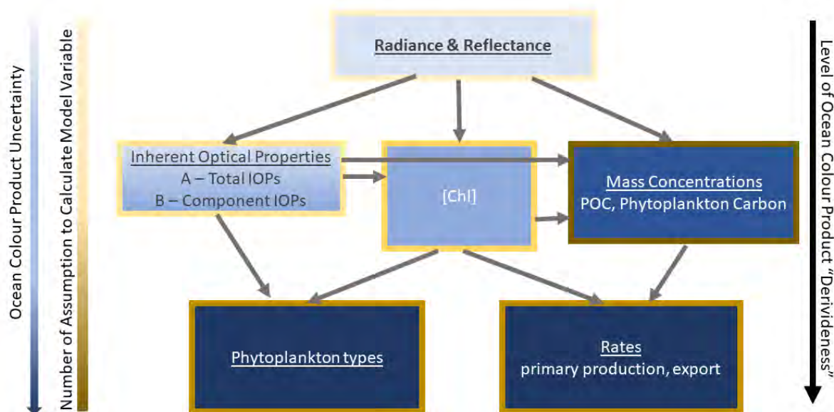
Figure 4.1. Schematic depicting uncertainties and level of “derivedness”. For Ocean Colour products, uncertainty is coloured in blues, with darker colours suggesting more uncertainty. Assuming radiance and reflectance are the least derived ocean colour, the vertical position (tier) of each box depicts how many levels of products are used to derive it. The gray arrows indicate which products are used to derive which other products. For instance, Chl-a can be derived either from radiances and reflectance or from IOPS. In general, the more derived the product is, also the more uncertain it is. The brown colours surrounding the boxes indicate the level of assumptions needed to calculate the variable in the model. Most models follow carbon, so phytoplankton carbon is one of the most basic variable. IOPS and reflectance require the most assumptions in the model to calculate.
