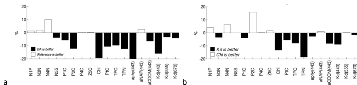
Figure 6.2. a) Skill of K_d(443) assimilation in estimating the L4 data: The bars represent the percentage differences between RMSE of the assimilation (DA) versus the reference (ref) simulation; b) Skill for K_d(443) versus chlorophyll (chl) assimilation in estimating the L4 data: The bars represent the differences between the RMSE obtained in the two assimilative runs. The x-axis lists model variables: N1P: phosphate; N3N: nitrate; N4N: ammonium; N5S: silicate; P1C: diatom carbon biomass; P2C: nanophytoplankton; P3C:
