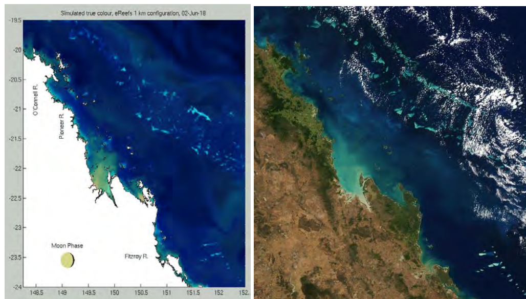
Fig. 4.3 Comparison of simulated (left) and observed (right) true colour in the complex coastal waters of the Great Barrier Reef on 2 June 2018. Simulated true colour (left) obtained from simulated remote-sensing reflectance at 645, 555 and 470 nm of the ~1 km resolution eReefs simulation ( www.eReefs.info , Baird et al., 2016). The ~250 m observed true colour (right) is from the MODIS Aqua sensor processed using Worldview. Both images are generated using the NASA true-colour processing algorithm. Worldview uses MODIS Bands 1, 4, and 3, respectively corresponding to the red, green, and blue range of the light spectrum, assigned to the red, green, and blue channels of a digital image. The images include a brightening factor that depends on the graphics package rendering the image, and have been approximately matched.
