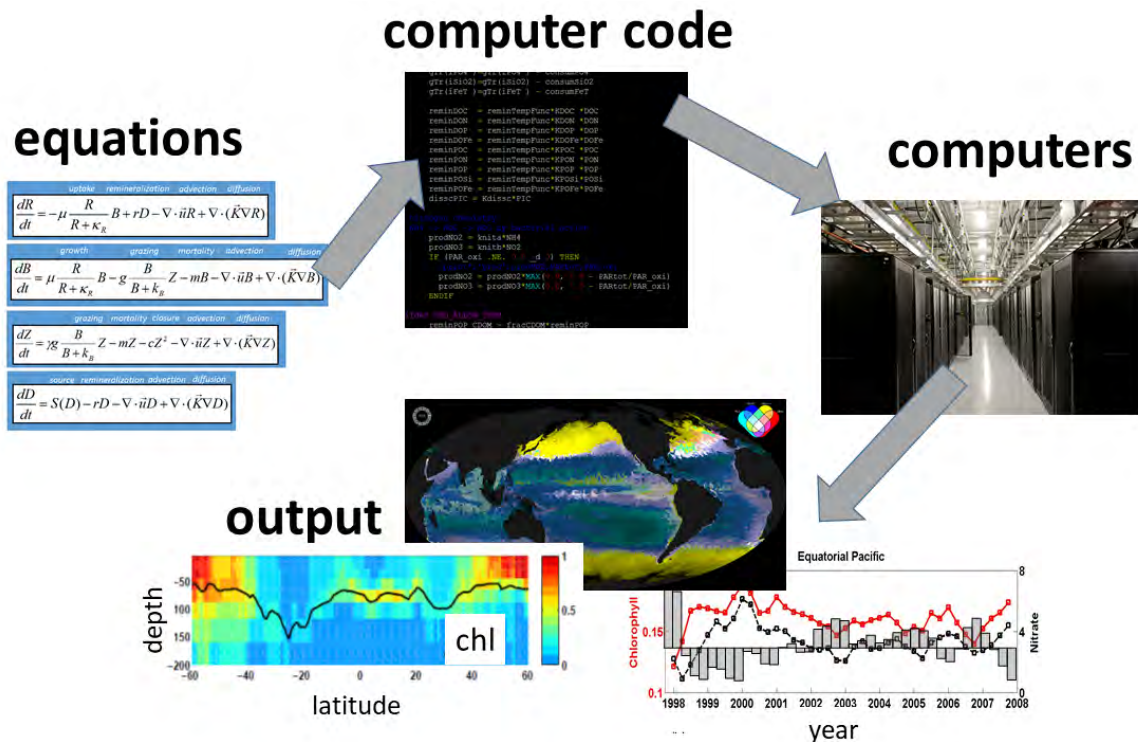
Figure 3.3: Schematic on developing and using a numerical model. First the set of appropriate equations are devised for all model state variables (e.g. for each box of the NPZD model, see Fig 3.2). Next the equations are written as computer code that is made into an “executable file” that a computer (or cluster of computers) will run, output in terms of concentration of variables (such as biomass) are provided for analysis (and maps as displayed here). The model output is 3-dimensional and varies with time.
