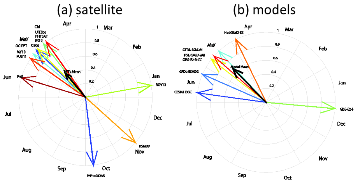
Figure 4.7. Comparison of satellite and modeled microplankton phenology in Longhurst (1998) North Atlantic Drift province. (a) Months of maxima of the satellite PFT algorithms; (b) Months of maxima of the models' diatom carbon biomass for the North Atlantic Drift Region. (Modified from Kostadinov et al. 2017).
