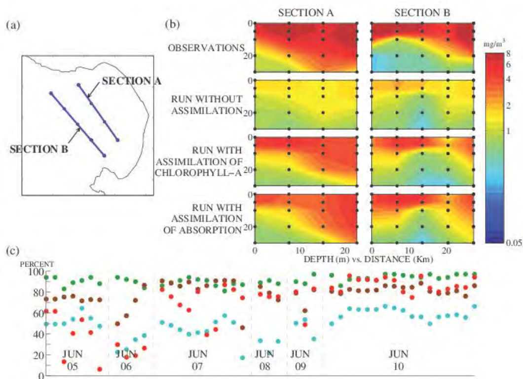
Figure 6.8. (a) – locations of water samples stations A and B; (b) Comparisons of observed (sections A and B) and model predicted subsurface chlorophyll distributions at water sample locations; (c) Observed and model-predicted fractions of diatoms to the whole phytoplankton populations at water samples locations: green – HPLC observed fractions, blue light – run without assimilation of bio-optical properties, brown – run with assimilation of satellite Chl data; red- run with assimilation of absorption due to phytoplankton.
