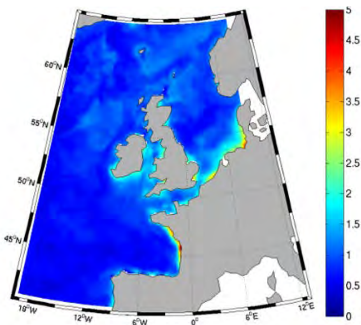
Figure 3.11. Regional Model. Surface chlorophyll concentration [ \text{mg m}^{-3} ] from the simulation of a regional model of the North East Atlantic: average value in the years 1998-2009 (adapted from Ciavatta et al., 2016)
