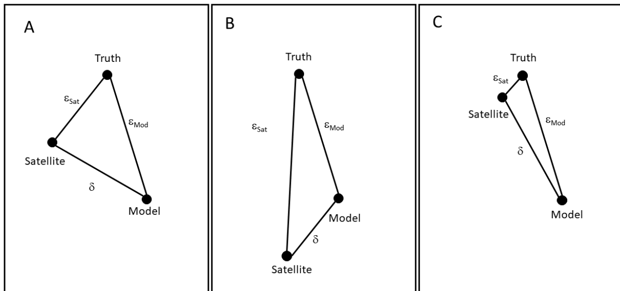
Figure 5.1: Truth, error and misfit in comparing ocean colour estimates and models (Following Lynch et al. , (2009)). Both satellite-based measurements and simulations are approximations of the true ocean state (e.g., chlorophyll), with errors characterized by \epsilon_{Sat} and \epsilon_{Mod} , respectively. When assessing model predictions, one is ultimately interested in \epsilon_{Mod} , but the true state of the ocean cannot be known exactly. One must instead use the misfit ( \delta ) between the model and satellite-based estimates. The panels illustrate the implications of this for three different levels of satellite accuracy. Panel A, shows a case where both model and satellite estimates have significant uncertainty, but the satellite is slightly more accurate. In this case, perhaps typical of chlorophyll in open ocean regions [Gregg and Casey, 2004], \delta and \epsilon_{Mod} are similar: the measure of skill provided by the comparison with satellite is a reasonably robust measure of skill relative to the true ocean state, but should still be viewed with some caution. In Panel B, both the satellite estimate and the model are subject to large uncertainties. This case is comparable to skill assessments in the coastal ocean [Ciavatta et al. , 2011], or comparing against primary production [Carr et al. , 2006; Friedrichs et al. , 2009] and the misfit \delta relative to any single NPP algorithm may not be a good approximation of \epsilon_{Mod} . Finally, panel C represents a case where the satellite estimate is an excellent measure of the ocean state such that there is only a small difference between \delta and \epsilon_{Mod} .
