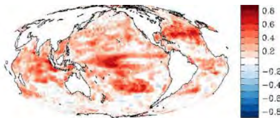
Figure 5.8: Anomaly correlation coefficients between ESM2M-COBALT simulated chlorophyll and GlobColour from a simulation integrating COBALT dynamics with physical data assimilation [ Park et al. , 2018]. Anomaly correlation coefficients are based on data from 1997-2017. The monthly chlorophyll climatology was removed before calculating anomalies, thus focusing the comparison on monthly anomalies rather than the monthly mean pattern.
