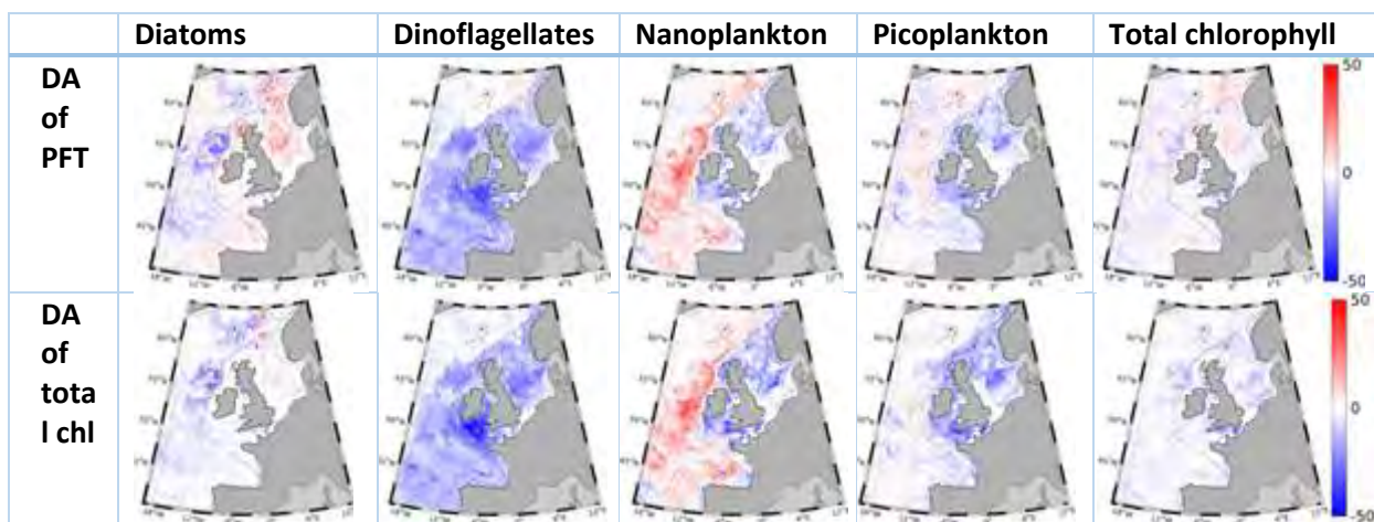
Figure 6.5. Skill of the reanalysis in simulating the ocean-colour plankton functional types. The maps show the percentage differences (%) between the data-to-output root-mean square-deviation (RMSD) of the PFT assimilation versus the reference simulation without assimilation (1 st row) and versus total chlorophyll assimilation (2 nd row). Negative values indicate that the RMSD of PFT assimilation is lower than the RMSD of the alternative simulation. The dotted lines indicate the 50 m and 200 m isobaths.
