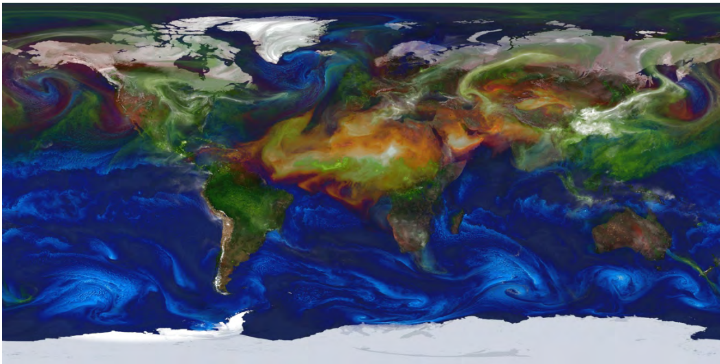
Figure 2.3. Global aerosol model distribution, where the colour-coded aerosol plumes indicate the aerosol type. Red shaded regions indicate presence of dust, blue is sea salt, green is carbonaceous aerosols (organic or black carbon), and gray is sulfates aerosols. (credit: NASA Global Modeling and Assimilation Office GEOS-5 Nature Run model)
