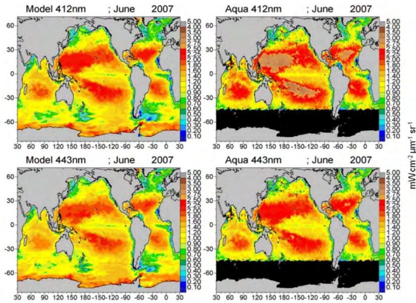
Figure 8.9: Model normalized water-leaving radiances for 412 and 443 nm compared to MODIS-Aqua radiances. Need journal permission.
