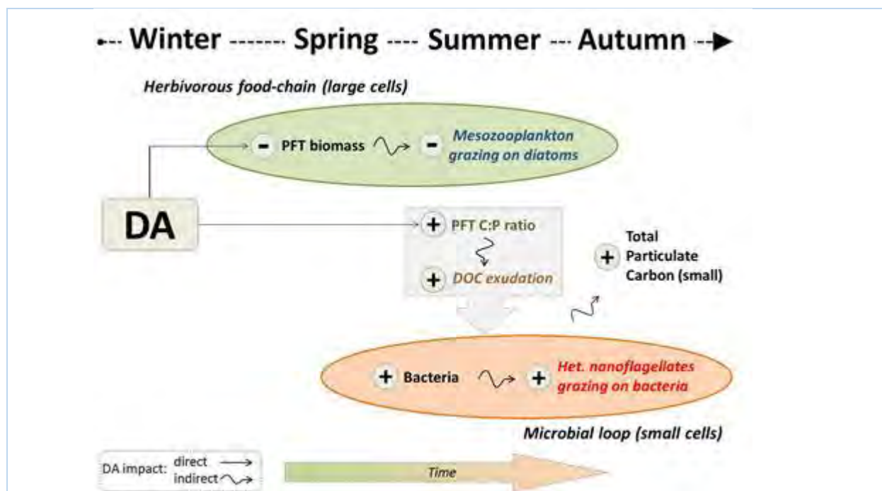
Figure 6.3. Scheme of the direct and indirect effects of data assimilation on the simulation of the trophic dynamic at L4. In the graphs, the bars represent the differences between selected carbon fluxes resulting from the data assimilation and reference simulations. The differences refer to winter (January-March), spring (April-June), summer (July-September) and autumn (October-December) 2006. The percentage values in brackets are the differences normalized by the mean seasonal values from the reference simulation
