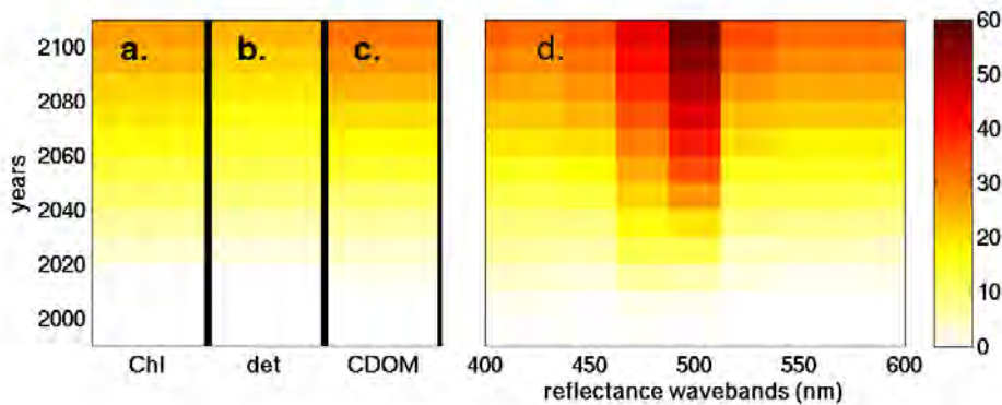
Figure 8.8. The amount of open ocean area that has statistically significant trend over the course of the 21 st century. (a) Chl-a is the sum of the 9 phytoplankton dynamically changing Chl-a (and similar to what would be
