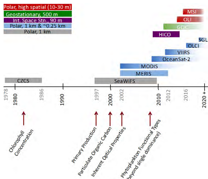
Figure 2.5. Current ocean colour mission lifetime with concurrent timeframe of major product developments. Faded gradient indicates missions in current operation. Note: OLI and MSI are instruments developed for terrestrial observations that have demonstrated success in some coastal applications.
