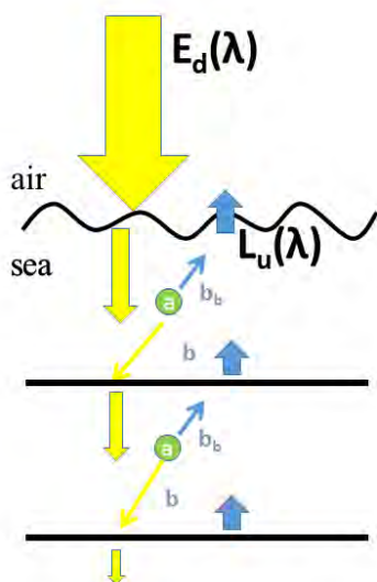
Figure 3.6. Schematic of light passage through the water column. Downward irradiance ( E_d ) is absorbed ( a ) by substances and particles (e.g. phytoplankton, detritus, CDOM). The light is also scattered in all directions, but includes a forward component ( b ) and a back component ( b_b ). This latter scattering leads to upwelling radiance ( L_u ). (See Chapter 2.1)
