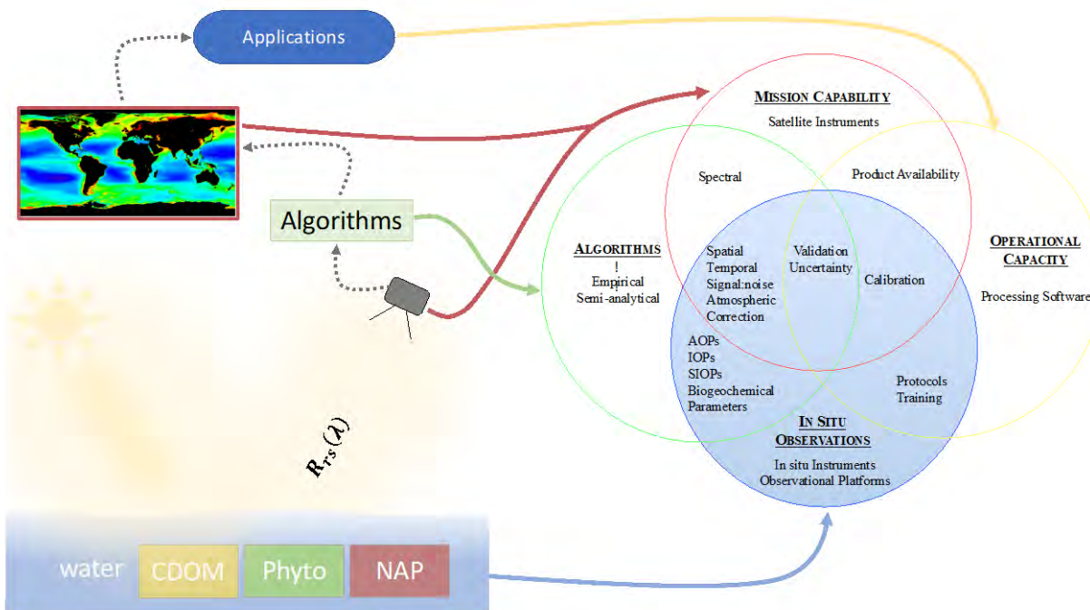
Figure 2.1. (Left) Schematic of path radiance from the sun, through the photic zone of the ocean, and through the atmosphere to a satellite radiometer. The optical constituents that influence ocean colour include pure water, chromophoric dissolved organic matter (CDOM), phytoplankton and non-algal particles (NAP). Satellite imagery is produced from atmospherically corrected spectral remote sensing reflectance, R_{rs}(\lambda) , with algorithms that connect satellite observations to optical, biogeochemical and water quality parameters. The inlaid image is mean chlorophyll a concentration obtained from MODIS-Aqua mission mean (2002-2017, https://oceancolour.gsfc.nasa.gov/ ). (Right) Venn diagram of the fundamental elements of ocean colour remote sensing, taken from Mouw et al. (2015).
