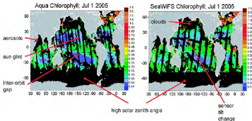
Figure 8.1: Daily ocean coverage by MODIS-Aqua and SeaWiFS, with sources causing data gaps identified
