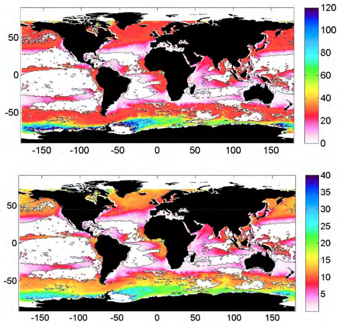
Figure 8.3: Maps of (top) uncertainty in bloom initiation date and (bottom) bloom peak date due to gaps in the satellite ocean colour time series (both in days). White areas do not have a distinct seasonal chlorophyll cycle (and therefore bloom initiation cannot be reliably calculated). (Figure modified from Cole et al. 2012)
