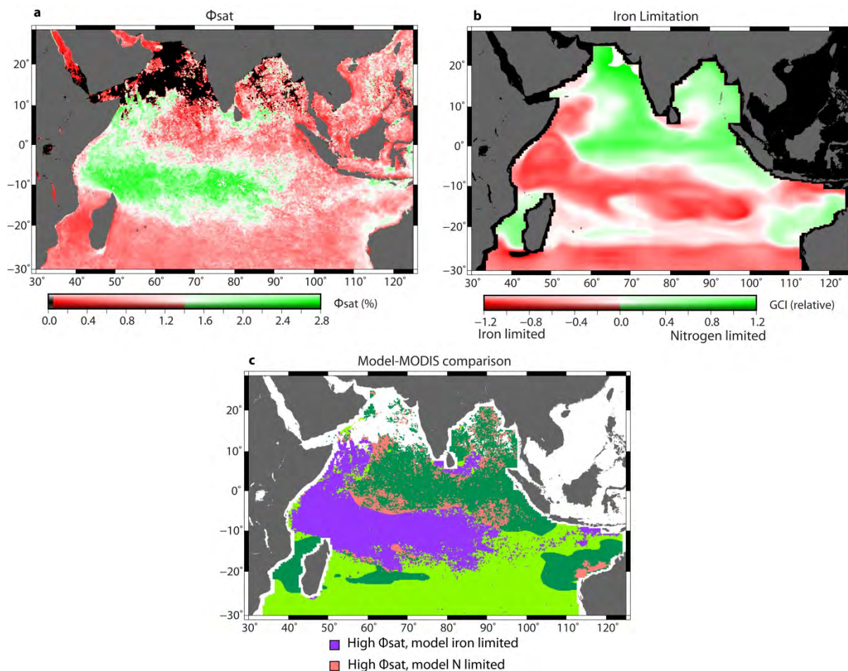
Figure 7.3: Indian Ocean (a) \phi_{sat} and (b) model-based growth constraint index (GCI) (Wiggert et al., 2006) for boreal summer (June–August). (c) State-space comparison of \phi_{sat} and GCI. (redrawn from Behrenfeld et al., 2009)
