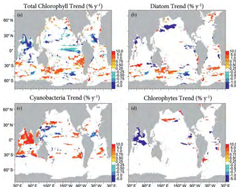
Figure 6.9. Reanalysis of the global ocean ecosystem by assimilating integrated ocean-colour time series of chlorophyll concentrations measured by SeaWiFS, MODIS, and VIIRS: Significant trends in a) total chlorophyll, b) diatoms, c) cyanobacteria, and d) chlorophytes over the period 1998–2015 (% y^{-1} ) [Gregg et al., 2017].
