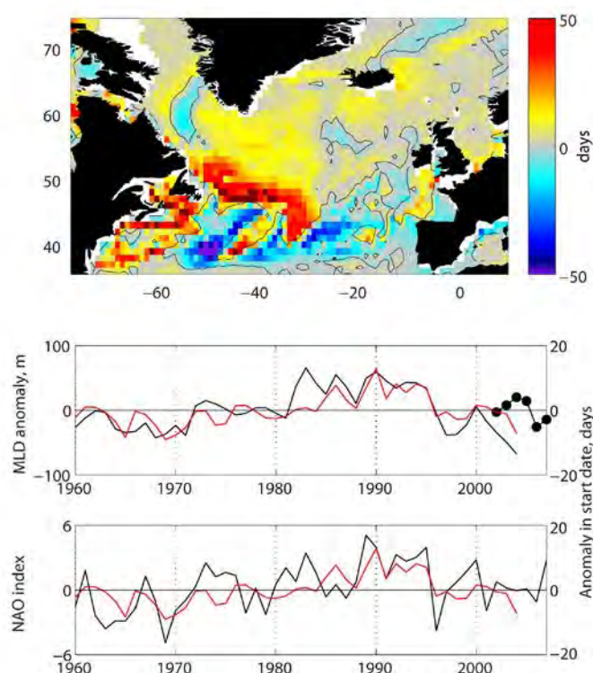
Figure 7.4. Top panel: difference in modelled bloom start date between the long-term mean (1960-2004) and a positive NAO phase (1998-1995), where positive values indicate a later bloom start in positive NAO phases. Middle panel: Time series of modelled subpolar bloom start date (red line), annual mean modelled MLD (black line) and Argo float-derived MLD (black dots). Bottom panel: Time series of modelled subpolar bloom start date (red line) and the NAO index (black line). (redrawn from Henson et al., 2009)
