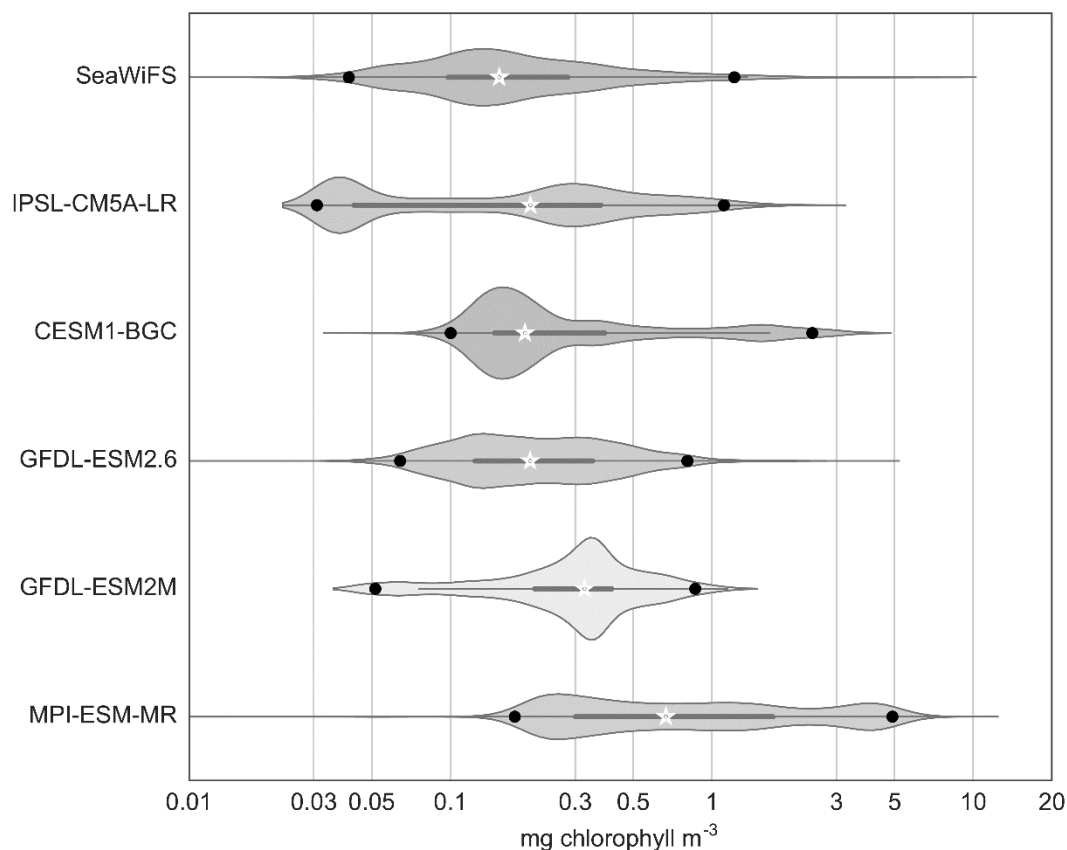
Figure 5.7: Violin plots comparing the probability distributions of annual mean chlorophyll from various global Earth System Models (ESMs) against chlorophyll estimated from SeaWiFS [figure adapted from Van Oostende et al., 2018 ]. The width of each violin is proportional to the number of points in each bin. Note that spatial agreement is not assessed in this comparison, only the distribution of chlorophyll values across the range of global values.
