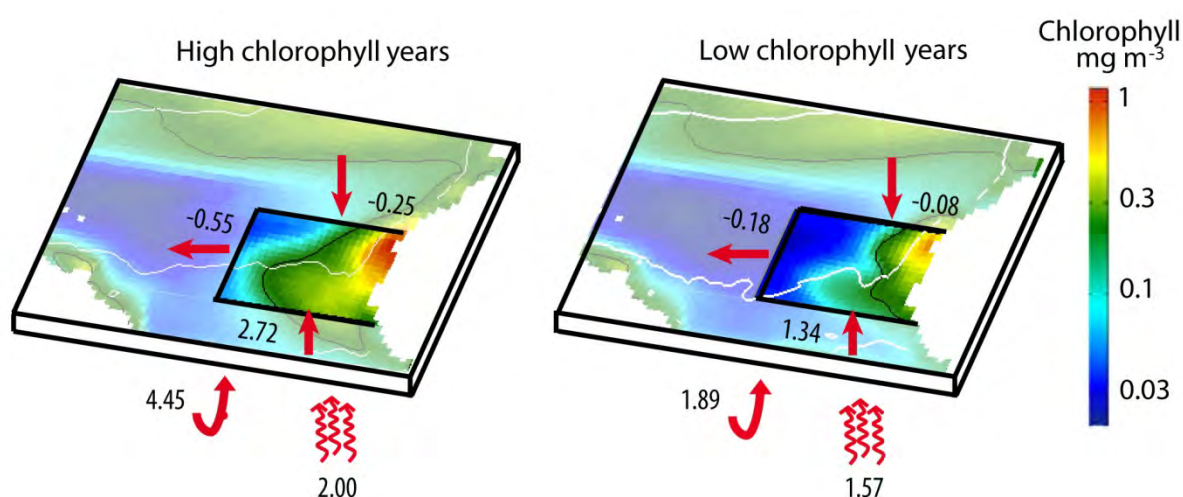
Figure: 7.1 Model results of nutrient supply to the upwelling region of the northeast Atlantic in contrasting high and low chlorophyll years. Solid arrows show the horizontal and vertical advective supply and curly arrows show the mixing term (all terms in 10^{-10} \text{ mol m}^{-2} \text{ s}^{-1} ). (redrawn from Pastor et al. 2013)
