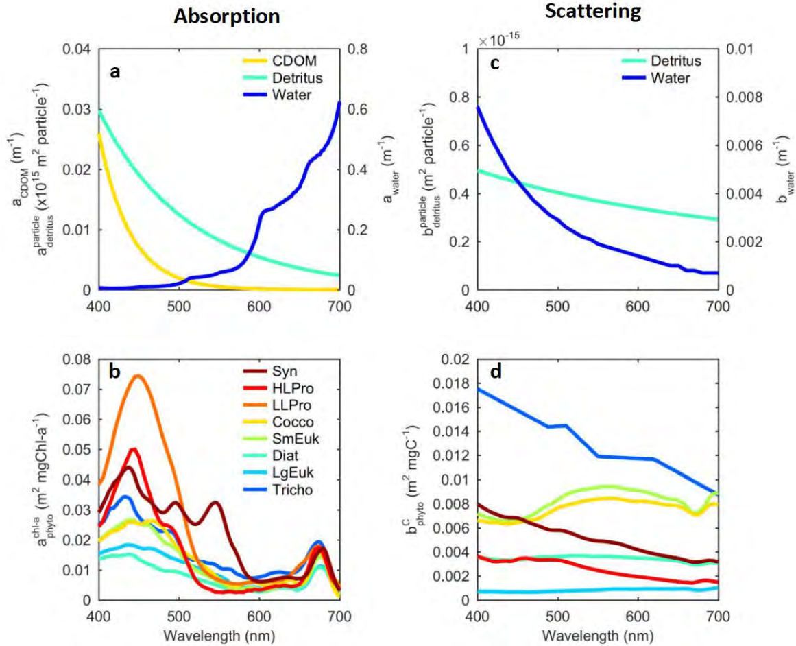
Figure 2.4. Spectral absorption and scattering of ocean optical constituents. Spectral absorption for a) water, chromophoric dissolved organic matter (CDOM), non-algal particles (NAP)/detritus, and b) various phytoplankton groups. Spectral scattering c) NAP/detritus, water, and d) various phytoplankton groups. The phytoplankton types were taken from Dutkiewicz et al. (2015) and include: Syn, Synechococcus ; HLPPro, Prochlorococcus ; LL- Pro, Prochlorococcus ; Cocco, Emiliania huxleyi ; SmEuk, Isochrysis galbana ; Diat, Thalassiosira weiss-flogii ; LgEuk, Prorocentrum micans ; Tricho, Trichodesmium sp. The phytoplankton optical characteristics were obtained for representative types in culture. Spectral a_{\text{CDOM}} are the observed average from several AMT transects (Kitidis et al. 2006). Adapted from Dutkiewicz et al. (2015).
