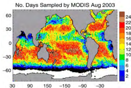
Figure 8.2: Number of days sampled by MODIS for August 2003. (From Gregg and Casey, 2007a). Need permission from journal
