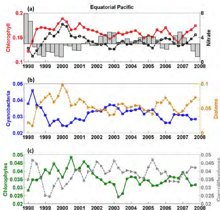
Fig 3.9 Hindcast Model. Temporal variation of nitrate and phytoplankton concentration in the Equatorial Pacific. Seasonal average (JFM, detrended, seasonal climatology removed and average added) of (a) chlorophyll a (mg chl a m -3 ) and nitrate concentration (μM). Shaded bars represent the Multivariate ENSO index (MEI), note that the MEI was scaled to fit the plot (MEI varied between -1.33 and 2.68 over the period 1998–2007). (b) Abundance of modelled cyanobacteria and diatoms (mg chl a m -3 ). (c) Abundance of modelled chlorophytes and coccolithophores (mg chl a m -3 ). Figure from Rousseaux and Gregg (2012). Need Journal permission
