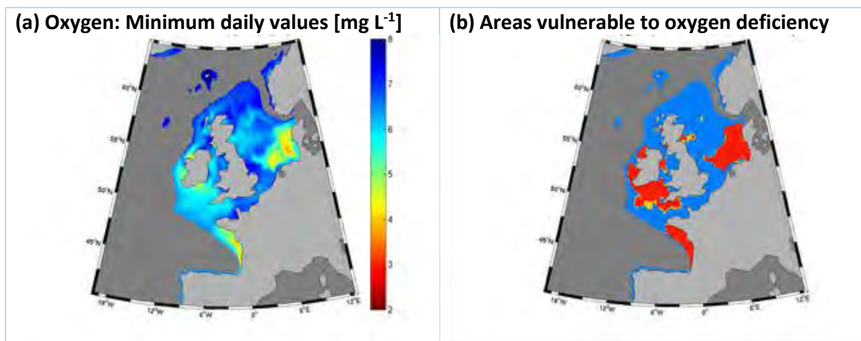
Figure 6.10 Reanalysis of biogeochemical indicators in the North West European shelf (years 1998-2009) by assimilating an ocean-colour chlorophyll product with the Ensemble Kalman filter (100 ensemble members; Ciavatta et al., 2016): (a) Minimum daily values of dissolved oxygen simulated by the ensemble median at the bottom of the shelf and (b) map of the areas at risk of oxygen deficiency, i.e. with at least one daily value in 1998-2009 below the threshold of 6 \text{ mg L}^{-1} (OSPAR, 2013). In (b), yellow colour represent deficient areas at 1% confidence level (i.e. at least one member of the ensemble signals oxygen deficiency), red represents 100% confidence (all the one-hundred members signal deficiency).
