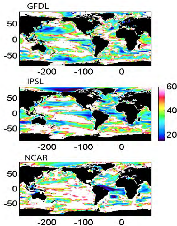
Figure 8.7: Number of years of continuous data required to distinguish a climate change-driven trend in chlorophyll concentration from natural variability, calculated for the GFDL, IPSL and NCAR models (IPCC A2 scenario, 2001-2100). White areas indicate where the trend is not statistically significant. (Modified from Henson et al., 2010).
