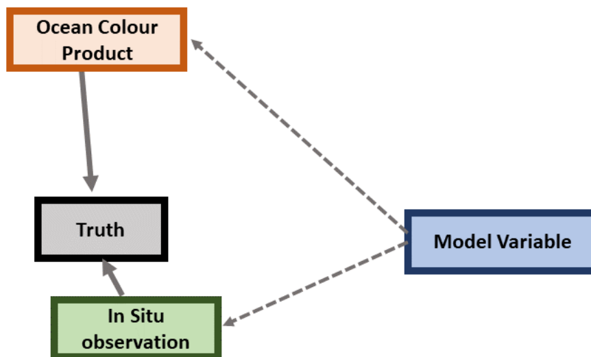
Fig 4.2. Schematic of uncertainties in in situ and ocean colour products. Truth (e.g. the actual Chl-a content at a location) can be measured in the field by several techniques (e.g. HPLC, fluoremetry, see Section 4.1.3) and there are several ocean colour products of Chl-a (e.g. reflectance ratios or semi-empirical methods, see Chapter 2.3.1). The length of solid arrows suggests the level of uncertainty of the measurements. Generally, in situ measurements are less uncertain than the ocean colour products. Model variables can be compared to either in situ or ocean colour products (usually both). It is important to remember that the two types of measurements are different, with different uncertainties and biases. Though often the quantities can be given the same “name”, they can have considerable mis-matches in what they actually capture.
