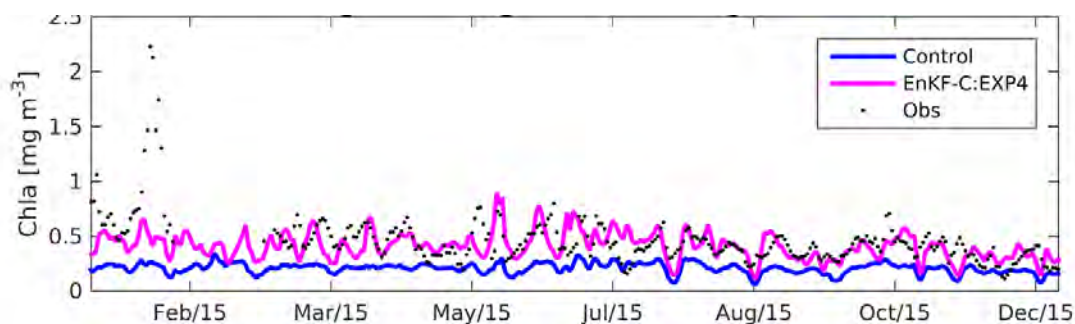
Figure 6.4. The comparison of the skill of the unassimilating (control) run and the mean of the ensemble, quantified as a mean absolute percent error of the mismatch between the simulated and observed R_{rs} (top); comparison of the chlorophyll concentration measured by a moored fluorimeter (Obs), and the control and assimilating runs at one site (Double Cone off Airlie Beach, central Queensland) at 5 m depth.
