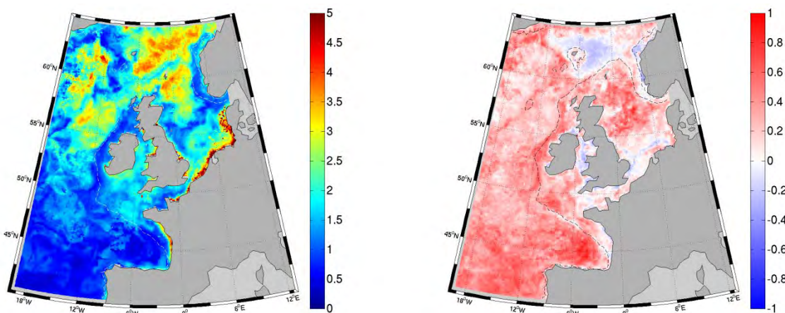
Figure 5.5: Skill assessment of a decadal reanalysis simulation of chlorophyll in the North East Atlantic in the year 1998-2009 (a) using the ocean colour product from ESA’s CCI programme. Root-mean-square-deviation (c) and Pearson correlation (d) defined in Table 5.1 were computed using time series of monthly data at each model grid point.
