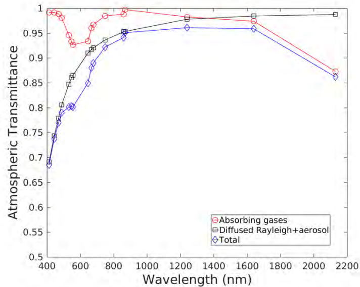
Figure 2.2. Atmospheric transmittance and spectral absorption and scattering of atmospheric constituents for solar zenith angle of 30^\circ , sensor zenith of 20^\circ and relative azimuth of 140^\circ . These are moderate spectral resolution data, so some spectral features may not be fully represented. The water vapor concentration is 0.95 cm and ozone is 355 DU and average climatology \text{CO}_2 , \text{CH}_4 , \text{N}_2\text{O} , and \text{O}_2 . The aerosol optical depth is 0.1 at 869 nm with a 0.8 Ångström coefficient.
