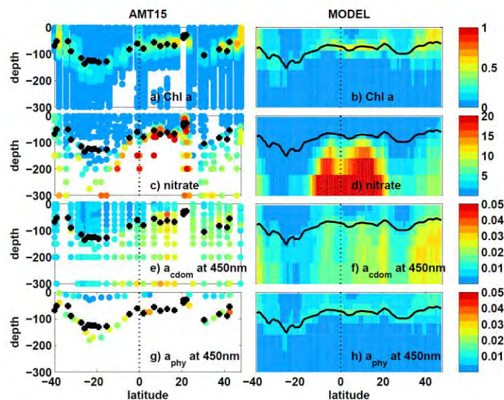
Fig 4.4. Model, observations comparisons along a transect through the Atlantic (Atlantic Meridional Transect 15). Observations on left are from (a) Chl-a; (c) nitrate; (e) absorption by CDOM, and (g) absorption by phytoplankton. The right column shows the model of Dutkiewicz et al (2015) (b) Chl-a parameterized as dynamical state variable for each of 9 phytoplankton types, and using Geider et al (1998) for C:Chl ratios; (d) nitrate as a state variable; (f) absorption by CDOM, where CDOM is a state variable and an exponential function relates absorption to CDOM concentration at different wavelengths; (g) absorption by phytoplankton, where absorption is linked to each of the 9
