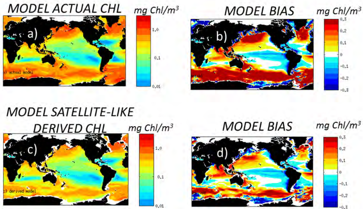
Figure 4.5: Comparison of model Chl-a to satellite-derived Chl-a. (a) Model annual average “actual” Chl-a. This is the explicit and dynamic Chl-a found from the phytoplankton in the model. (b) Bias between model and MODIS satellite derived Chl-a. Positive suggests that model over-estimates the Chl-a found from the satellite measurements. (c) product using the blue-green reflectance ratio and a 4 th order polynomial to estimate Chl-a in the manner used in satellite products (e.g. NASA OC4). (d) Bias between model “satellite-like derived” Chl-a and the MODIS-derived Chl-a.
