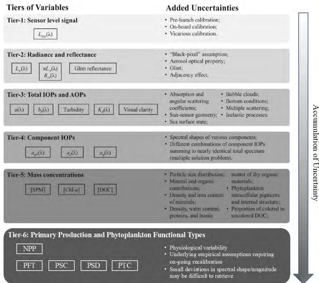
Figure 2.8. Tiers of satellite-derived products and associated uncertainties introduced at each tier. The list of products is representative, but not exhaustive. Adapted from Zheng and DiGiacomo (2017).
