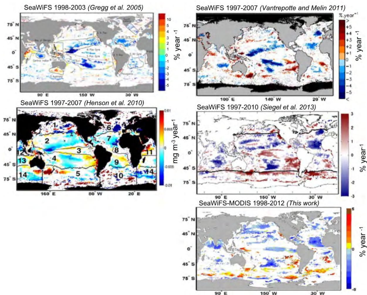
Figure 2.10. Comparison of five representations of chlorophyll trend maps in unit of percent per year (except middle left which is \text{mg m}^{-3} \text{ yr}^{-1} , from Gregg and Rousseaux, 2014).
