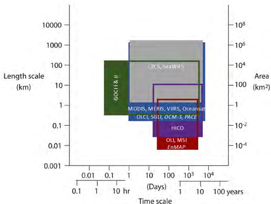
Figure 2.6. Spatial and temporal resolution of heritage, current and planned ocean colour satellite sensors. Planned sensors and missions are italicized. Note: OLI and MSI are instruments developed for terrestrial observations that have demonstrated success in some coastal applications. Adapted from Mouw et al. (2015).
