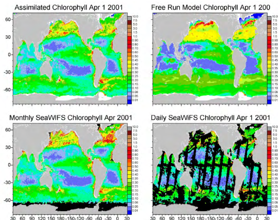
Figure 6.1: Comparison of chlorophyll ( \text{mg m}^{-3} ) for April 1 st , 2001 from (top left) the assimilation model, (top right) the free-run, (bottom left) the monthly SeaWiFS chlorophyll for April 2001 and (bottom right) the daily SeaWiFS Chlorophyll for April 1, 2001.
