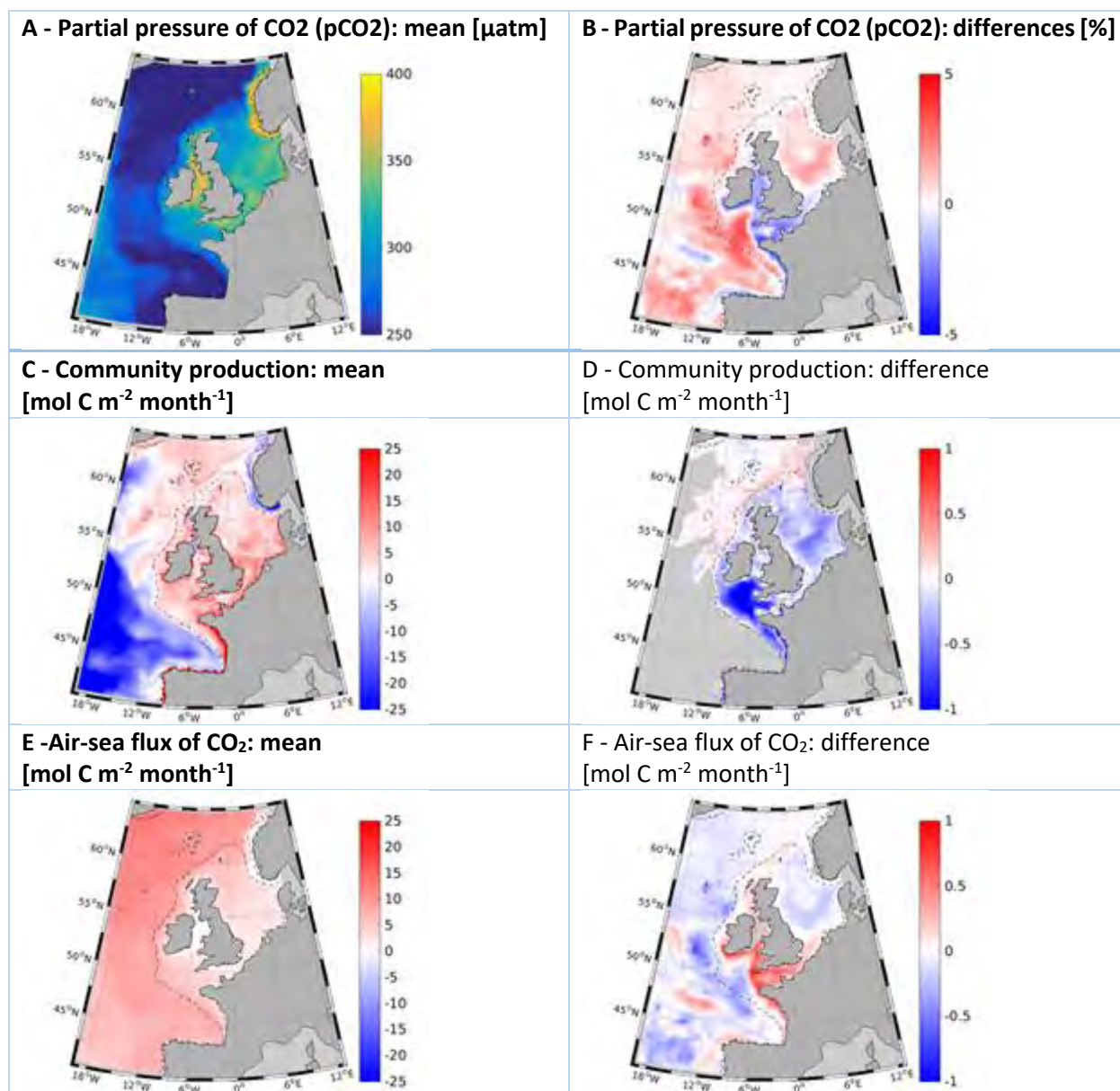
Figure 6.7. Reanalysis of pCO 2 (A and B; the partial pressure of CO 2 ), of the net community production (C and D; the difference between the primary production and the respiration of phytoplankton, bacteria, and zooplankton) and of the CO 2 air-sea flux (E and F, positive values indicate atmospheric CO 2 sink). Mean values in the years 1998-2003 (A, C, E), and difference between the reanalysis and reference mean values (B, D and F). For the net community production, the difference was computed in the areas where both the reanalysis and reference means are positive, i.e. in the autotrophic areas of the study region. The reanalysis decreased the bias and the absolute errors of pCO 2 estimates (Figure 6.6) because it decreased their high reference values in the Irish Sea and in the English Channel (A and B), while it augmented the low values in the Bay of Biscay and in the Celtic Sea (A and B). This is due to indirect assimilative changes in the carbon fluxes (i.e. a decrease of the net community production in the Celtic Sea driven by the decreased plankton biomass (C and D). As a relevant consequence, also the simulated air-sea fluxes of carbon dioxide changed in the reanalysis (E and F), following the patterns of its driver pCO 2 (A and B).
