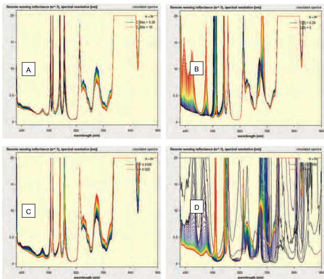
Figure 10: Spectral resolution for (A) TSM range 0.2 – 10.0 mg/l, (B) CHL range 0.2 – 5.0 \mu\text{g/l} , (C) S_{\text{CDOM}} range 0.010 – 0.020 \text{nm}^{-1} , (D) depth range 0.01 – 10.0 m.
