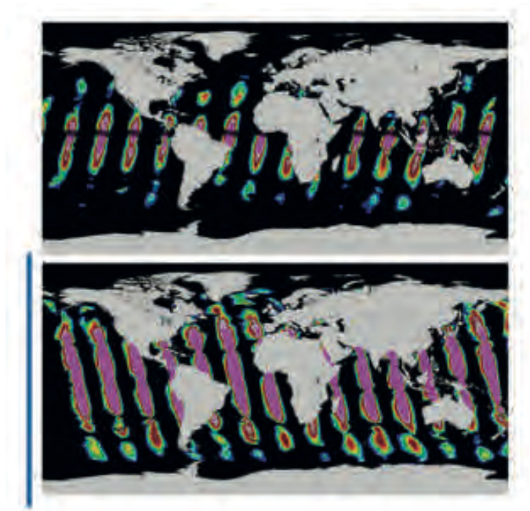
Figure 3.2 (after Meister et al., 2011) Illustration of how choosing sensor tilt (for SeaWiFS) significantly decreases the sun glint effects in the imagery. Global map of SeaWiFS (top) and MODIS Aqua (bottom) glint coefficients for March 22nd 2006. MODIS is not tilted. Glint coefficients larger than 0.005 in reflectance terms) are classified as high glint in NASA ocean colour processing and coloured pink in the images. Glint coefficients from 0.001 to 0.005 are classified as moderate glint and coloured red to white. The tilting of the SeaWiFS sensor significantly decreases the amount of data affected by sun glint.
