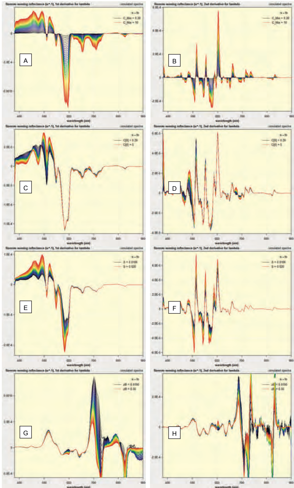
Figure 6: First (left column) and second (right column) derivatives of remote sensing reflectance for (A, B) TSM range 0.2 – 10.0 mg/l, (C, D) CHL range 0.2 – 5.0 \mu\text{g/l} , (E, F) S_{\text{CDOM}} range 0.010 – 0.020 \text{nm}^{-1} , (G, H) water depth range 0.01 – 0.50 m.
