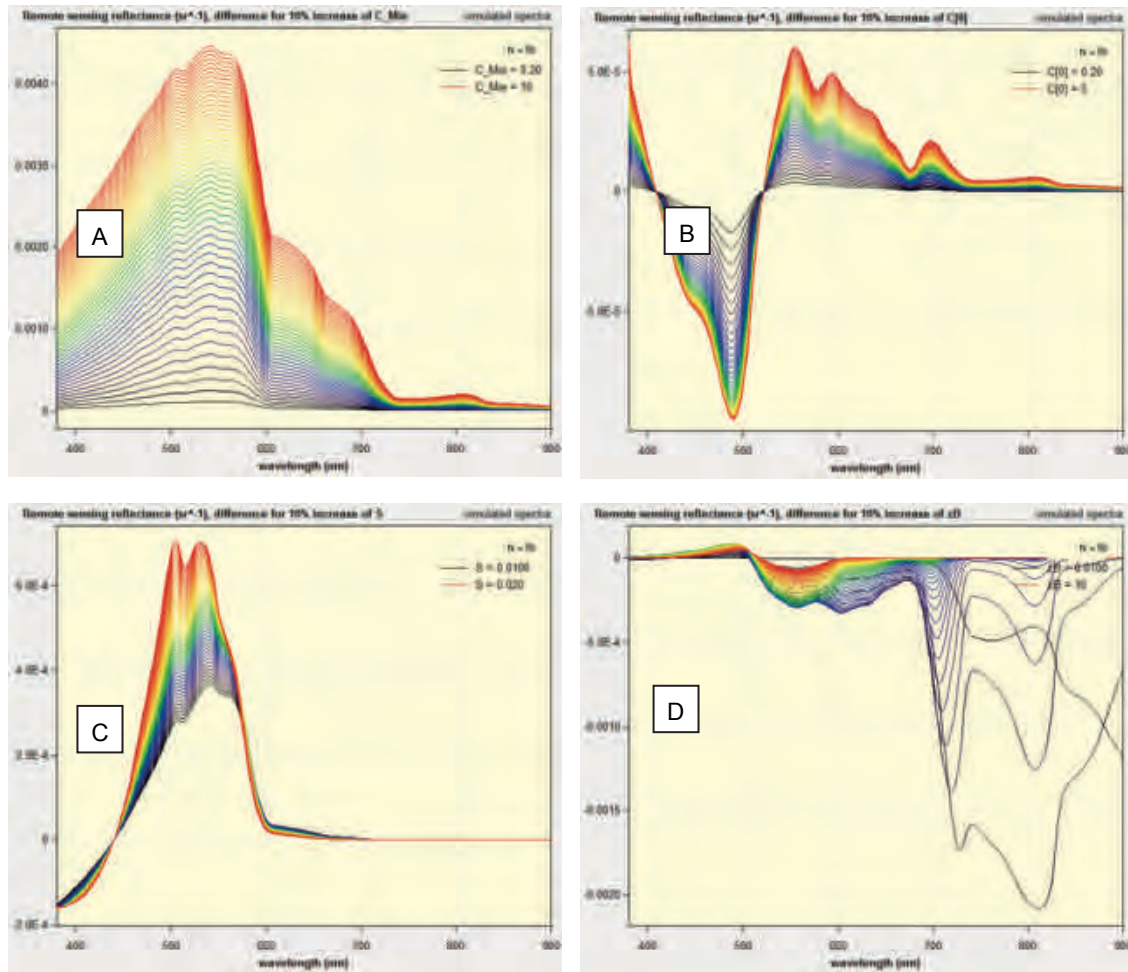
Figure 12: Changes of R_{rs} for 10% increase of (A) TSM in the range 0.2 – 10.0 mg/l, (B) CHL in the range 0.2 – 5.0 \mu g/l , (C) S_{CDOM} in the range 0.010 – 0.020 nm^{-1} , (D) depth in the range 0.01 – 10.0 m for bottom substrate of the seagrass Posidonia australis .
