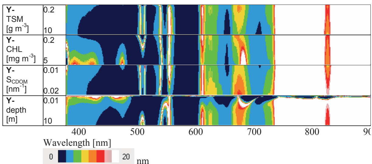
Figure 11: Spectral resolution required to resolve changes in reflectance (using NE\Delta R_{r,1} ) due to varying concentrations for scenario Y- .
