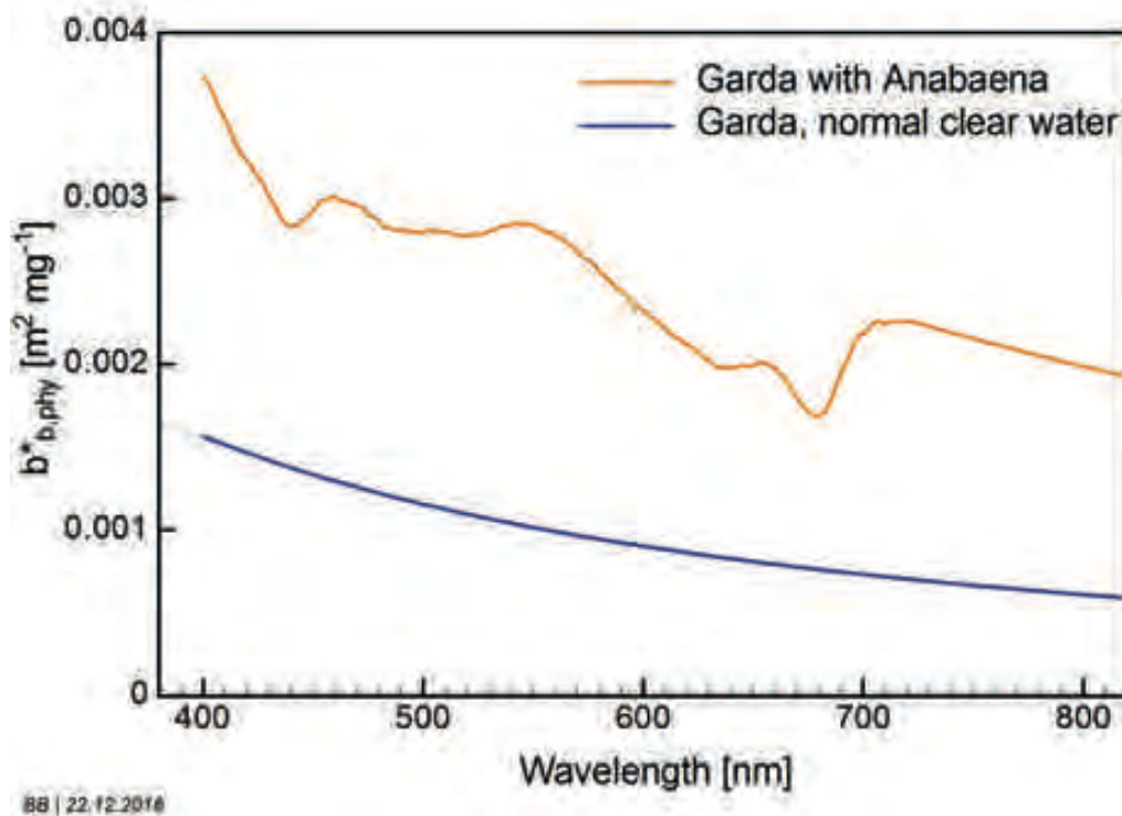
Figure 3: Specific backscattering coefficients of phytoplankton used for the simulations.
