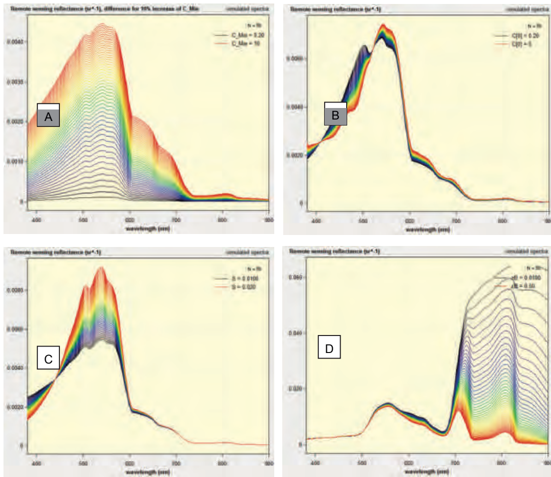
Figure 2.2 Remote sensing reflectance changes for (A) TSM range 0.2 - 10 mg/l, (B) CHL range 0.2 - 5 \mu g/l, (C) SCDOM range 0.010 - 0.020 \text{nm}^{-1} , (D) depth range 0.01 - 0.5 m with Posidonia cover of substratum
